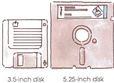
Figure 1-1 Software
