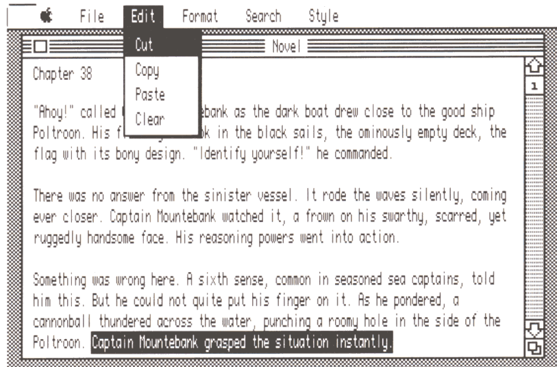
Figure 3-9 Cutting text
