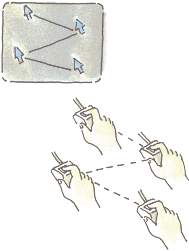
Figure 3-1 Pointing
