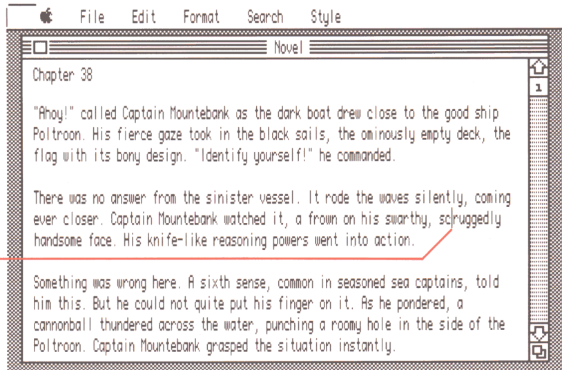
Figure 3-7 Inserting text
