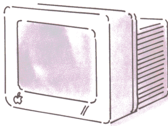
Figure 1-3 Peripheral devices
