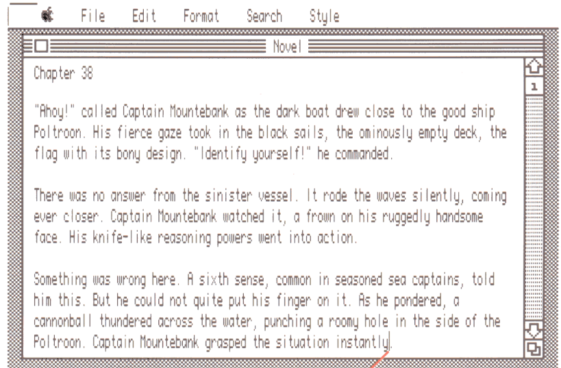
Figure 3-6 Insertion point
