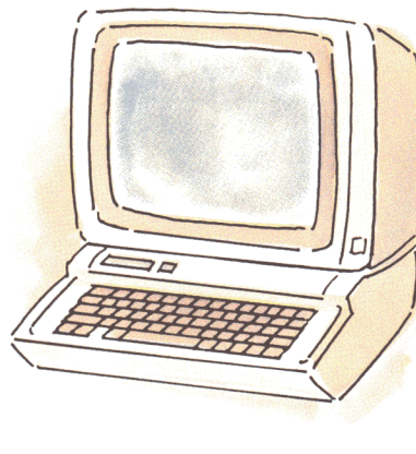
Figure C-2 Apple IIe
